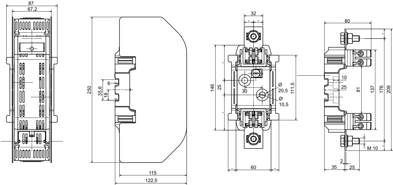
NH fuse-base for short NH fuse-links gPV, sizes 2, type PP with touch protection (dimensions in mm)
